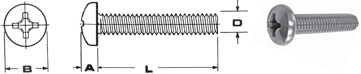
DIMENSION TABLE (INCHES)
