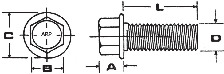
DIMENSION TABLE (INCHES) NOTE MANY SIZES ARE AVAILABLE IN TWO FLANGE DIAMETERS
