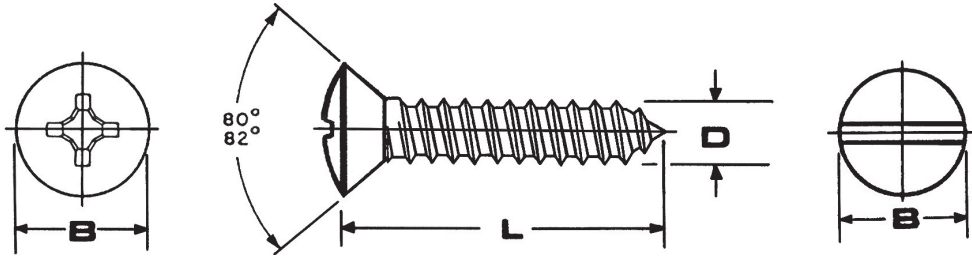
DIMENSION TABLE (INCHES)
