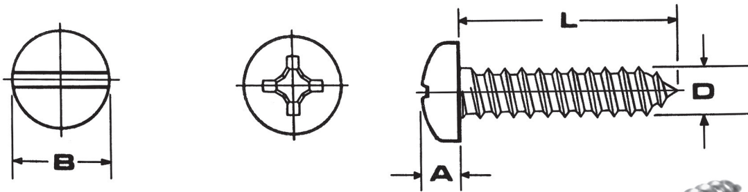
DIMENSION TABLE (INCHES)
