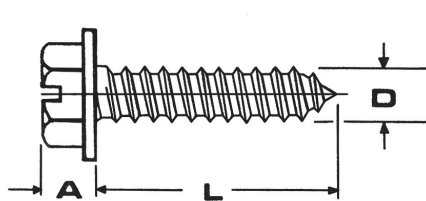
DIMENSION TABLE (INCHES)
