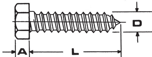
PLAIN INDENTED HEX DIMENSION TABLE (INCHES)
